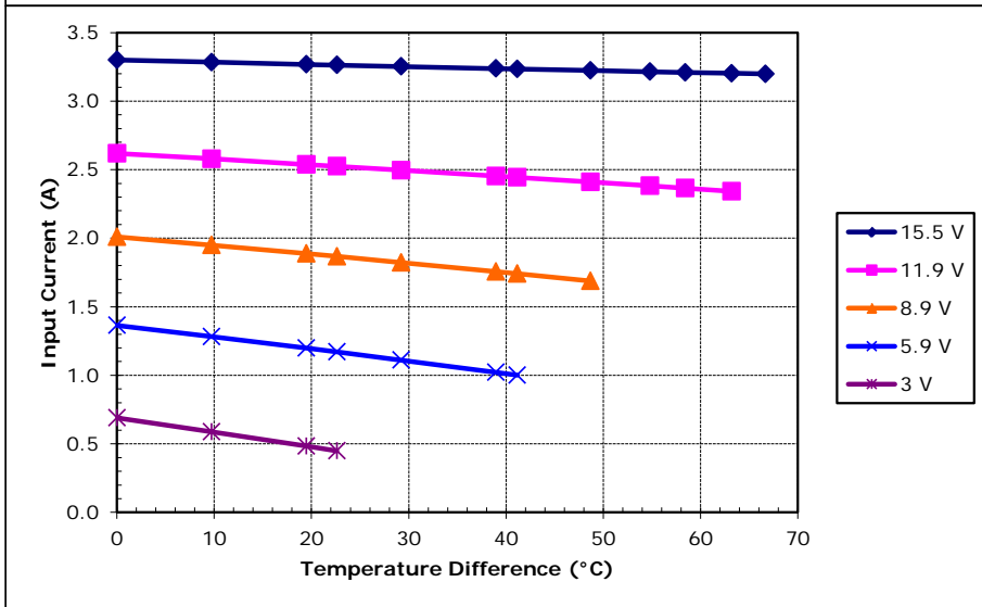
Potted TE-127-1.0-1.5 at a hot-side temperature of 30 °C
