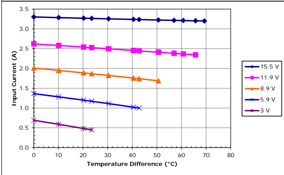
Unpotted TE-127-1.0-1.5 at a hot-side temperature of 30 °C
