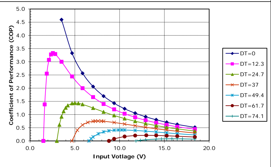
Unpotted TE-127-1.0-1.5 at a hot-side temperature of 70 °C
