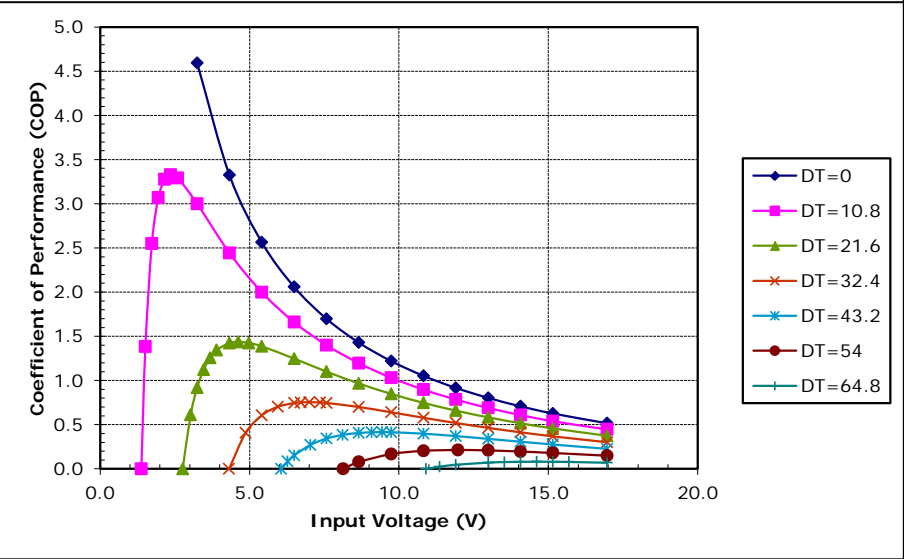
Potted TE-127-1.0-1.5 at a hot-side temperature of 50 °C
