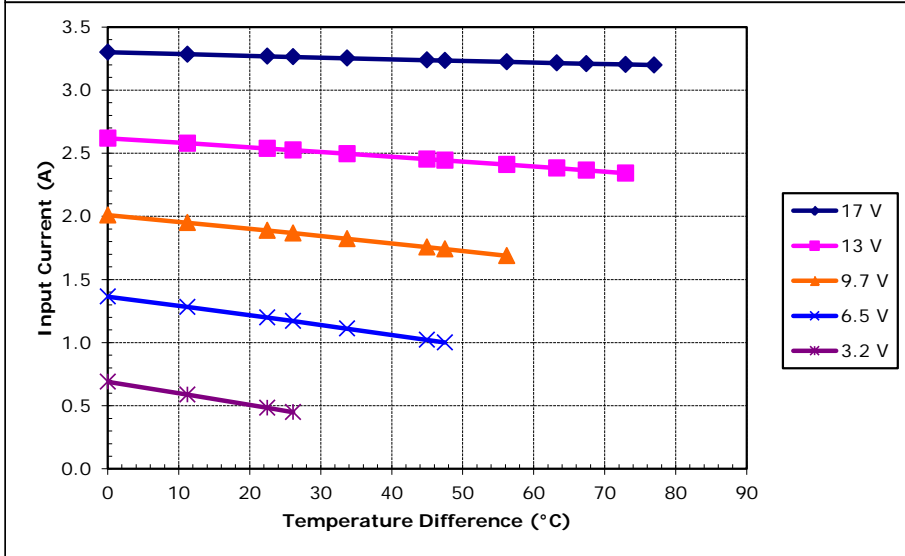
Unpotted TE-127-1.0-1.5 at a hot-side temperature of 50 °C
