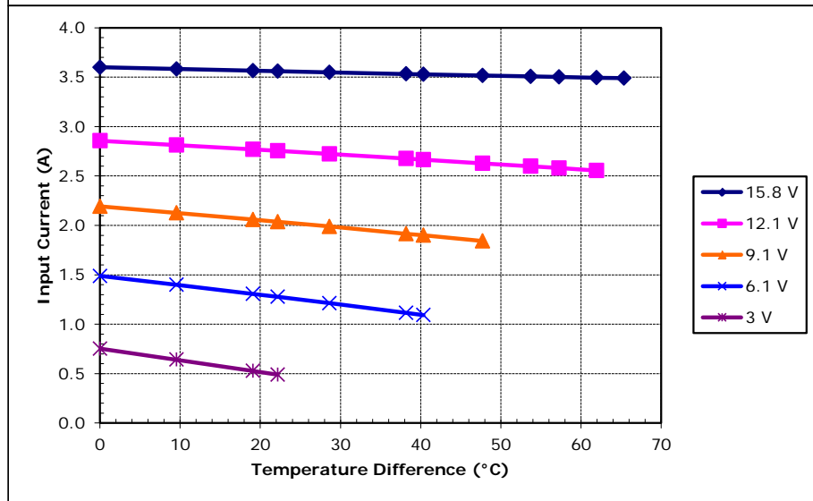
Potted TE-127-1.0-1.3 at a hot-side temperature of 30 °C
