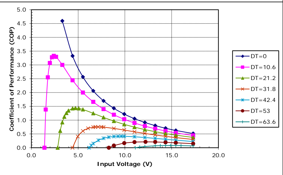
Potted TE-127-1.0-1.3 at a hot-side temperature of 50 °C
