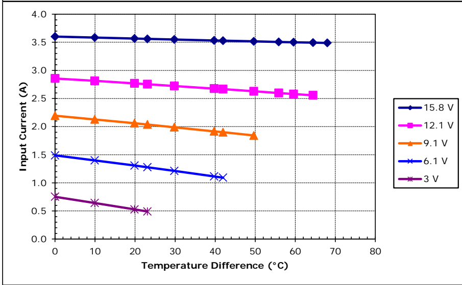
Unpotted TE-127-1.0-1.3 at a hot-side temperature of 30 °C
