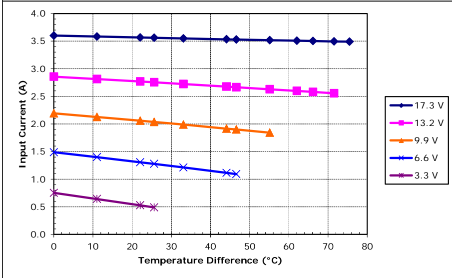
Unpotted TE-127-1.0-1.3 at a hot-side temperature of 50 °C
