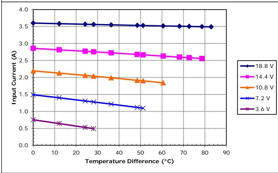
Unpotted TE-127-1.0-1.3 at a hot-side temperature of 70 °C
