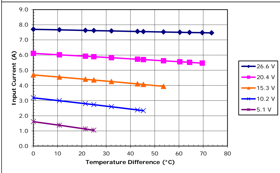
Potted HP-199-1.4-1.15 at a hot-side temperature of 50 °C
