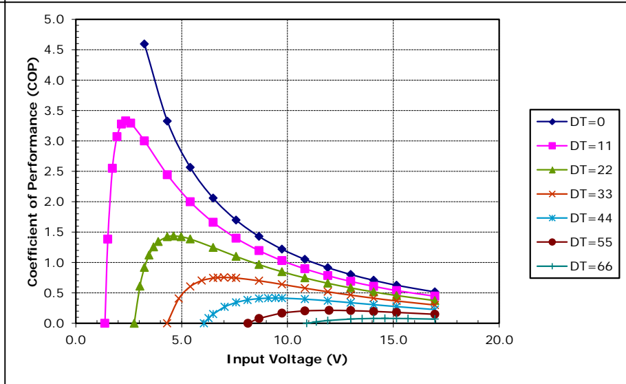
Potted HP-127-1.4-2.5-72 at a hot-side temperature of 50 °C
