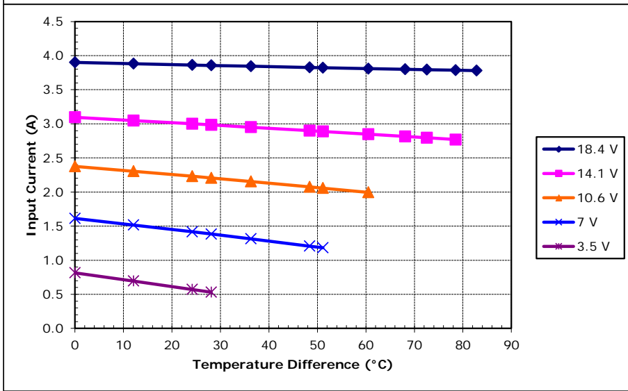
Potted HP-127-1.4-2.5-72 at a hot-side temperature of 70 °C
