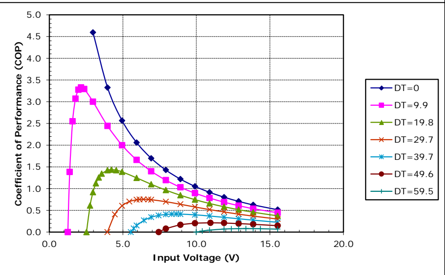
Potted HP-127-1.4-2.5-72 at a hot-side temperature of 30 °C
