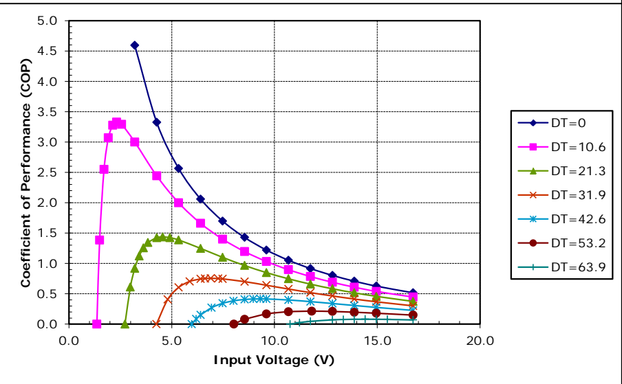
Potted HP-127-1.4-1.15-71 at a hot-side temperature of 50 °C
