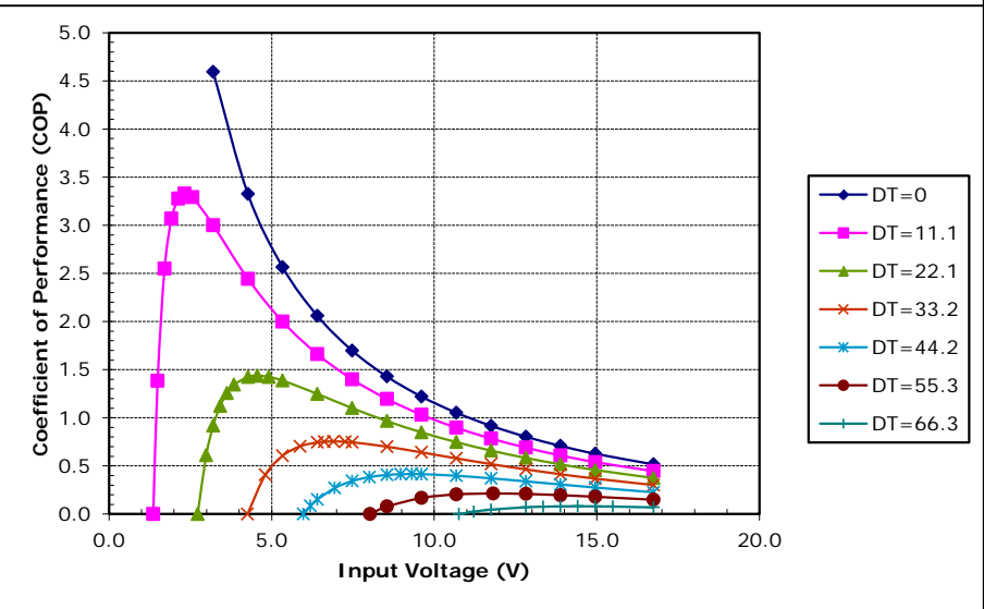
Unpotted HP-127-1.4-1.15-71 at a hot-side temperature of 50 °C
