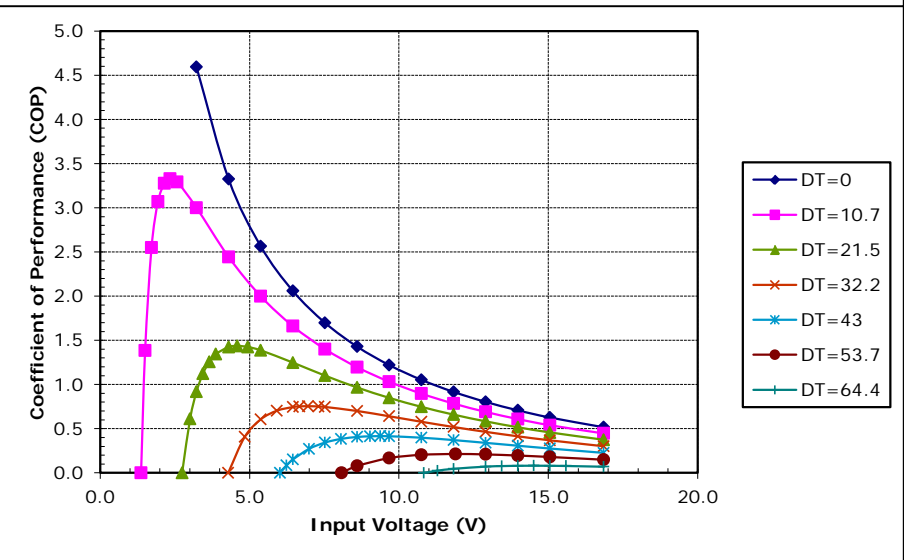
Potted HP-127-1.0-1.3-71 at a hot-side temperature of 50 °C
