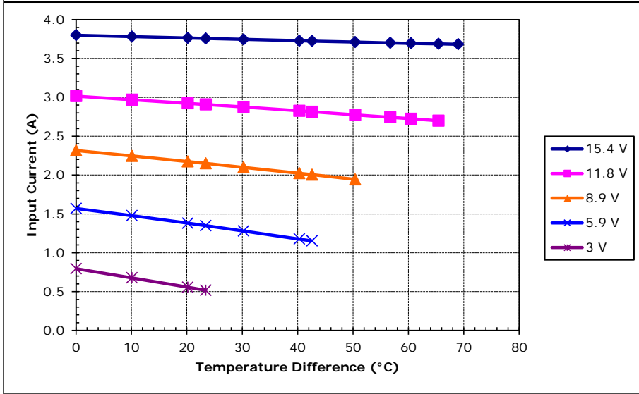
Unpotted HP-127-1.0-1.3-71 at a hot-side temperature of 30 °C
