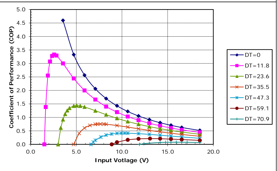
Unpotted HP-127-1.0-0.8 at a hot-side temperature of 70 °C
