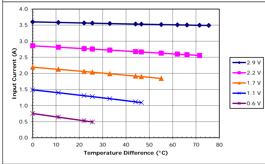
Unpotted CH-21-1.0-1.3 at a hot-side temperature of 50 °C
