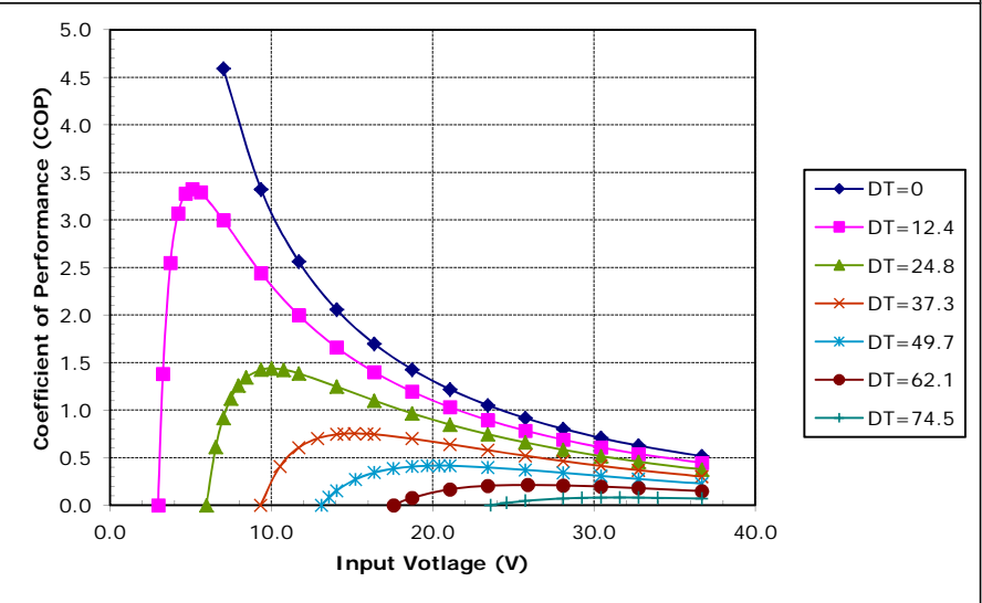
Unpotting RD-253-1.4-1.5 at a hot-side temperature of 70 °C
