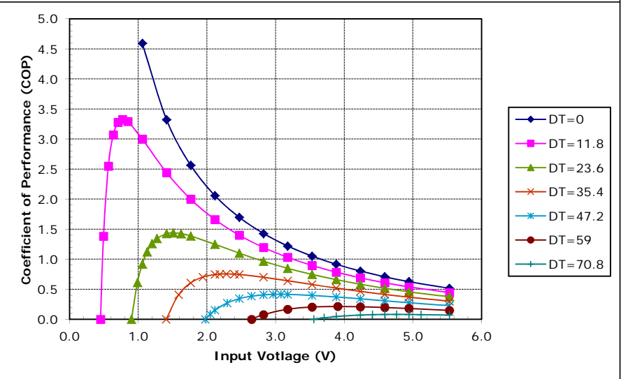
Unpotted CH-38-1.0-0.8 at a hot-side temperature of 70 °C
