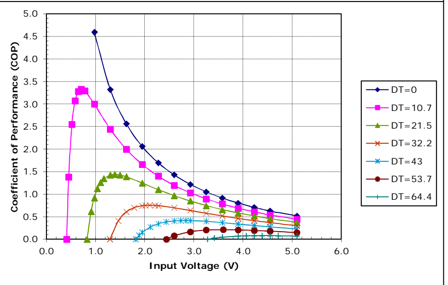
Unpotted CH-38-1.0-0.8 at a hot-side temperature of 50 °C
