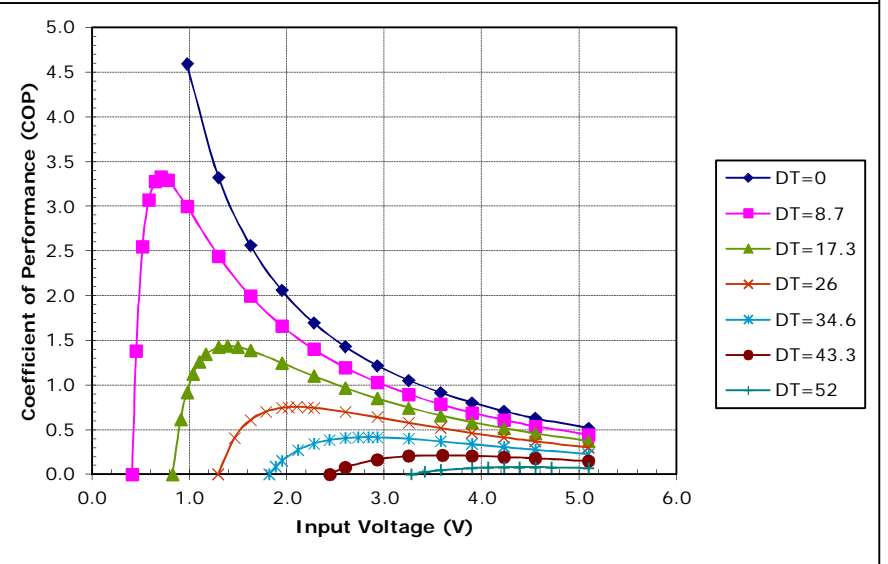
Potted CH-38-1.0-0.8 at a hot-side temperature of 50 °C
