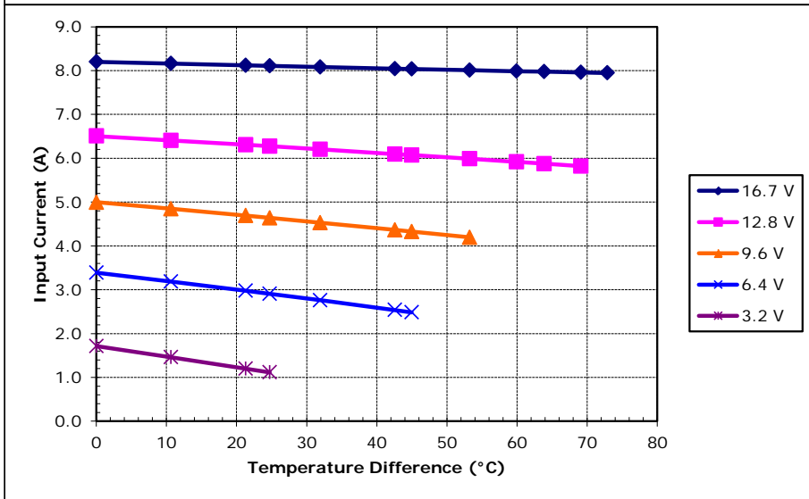
Potted VT-127-1.4-1.15-71 at a hot-side temperature of 50 °C
