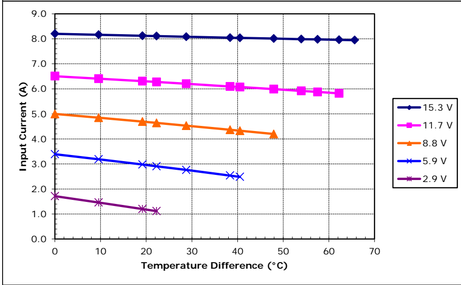
Potted VT-127-1.4-1.15-71 at a hot-side temperature of 30 °C
