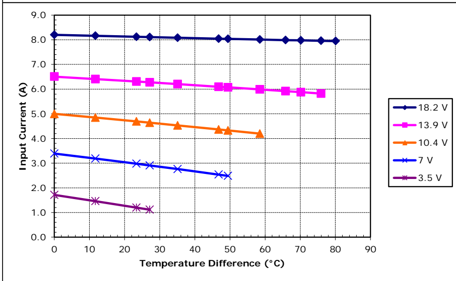
Potted VT-127-1.4-1.15-71 at a hot-side temperature of 70 °C
