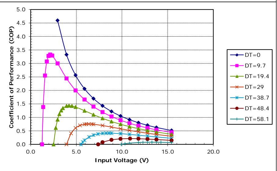
Potted VT-127-1.0-1.3-71 at a hot-side temperature of 30 °C
