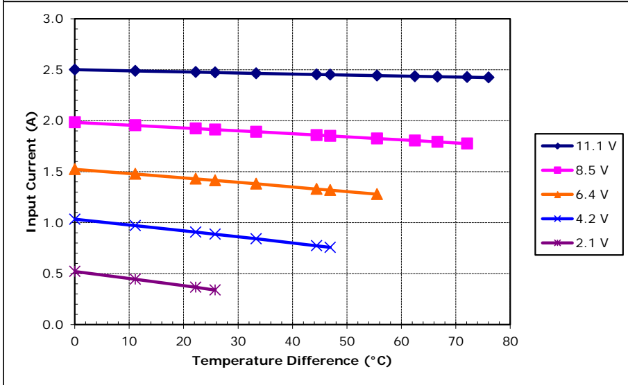
Potted TE-83-1.0-2.0 at a hot-side temperature of 50 °C
