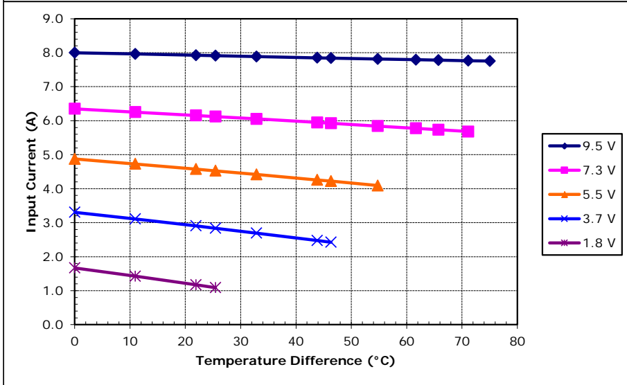
Potted TE-71-2.0-2.5 at a hot-side temperature of 50 °C
