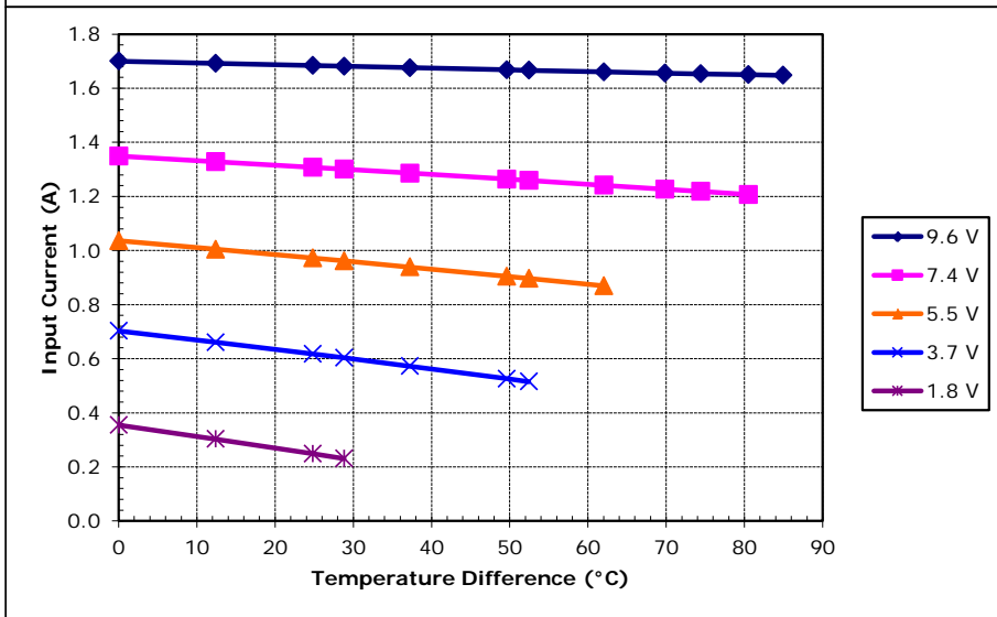
Unpotted TE-65-0.6-1.0 at a hot-side temperature of 70 °C
