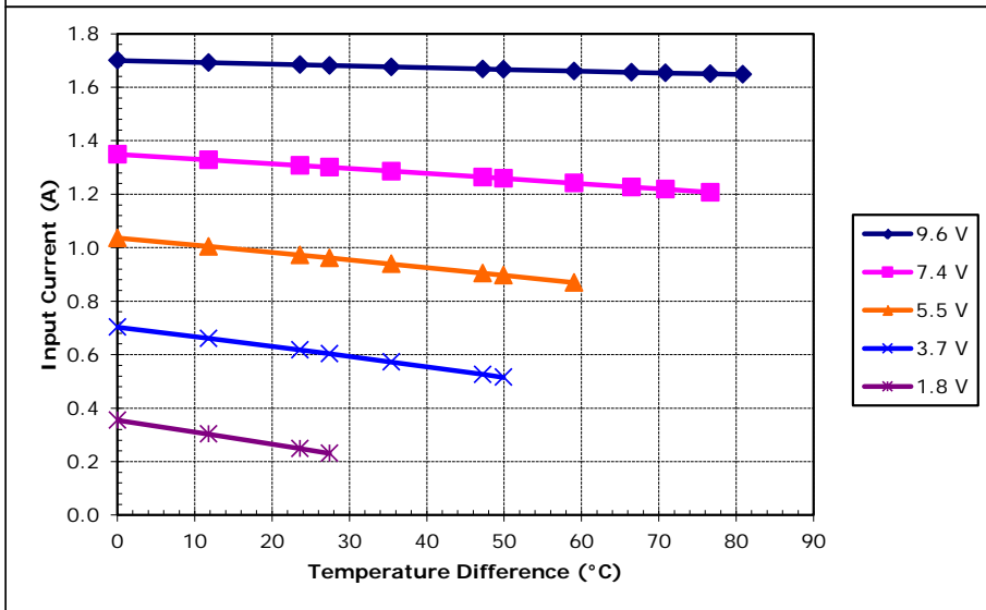
Potted TE-65-0.6-1.0 at a hot-side temperature of 70 °C
