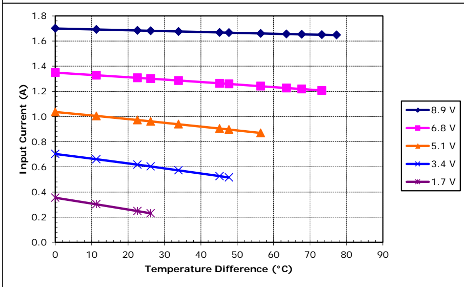
Unpotted TE-65-0.6-1.0 at a hot-side temperature of 50 °C
