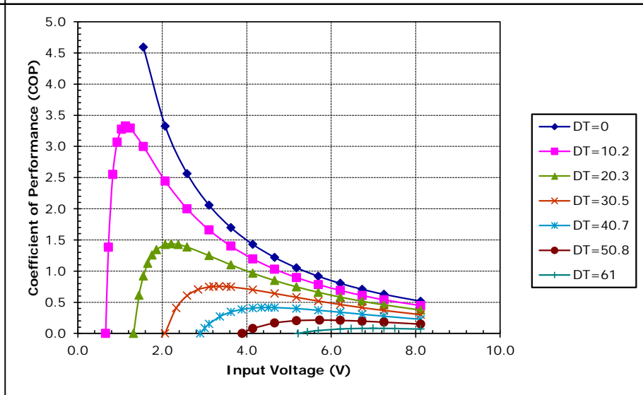
Unpotted TE-65-0.6-1.0 at a hot-side temperature of 30 °C
