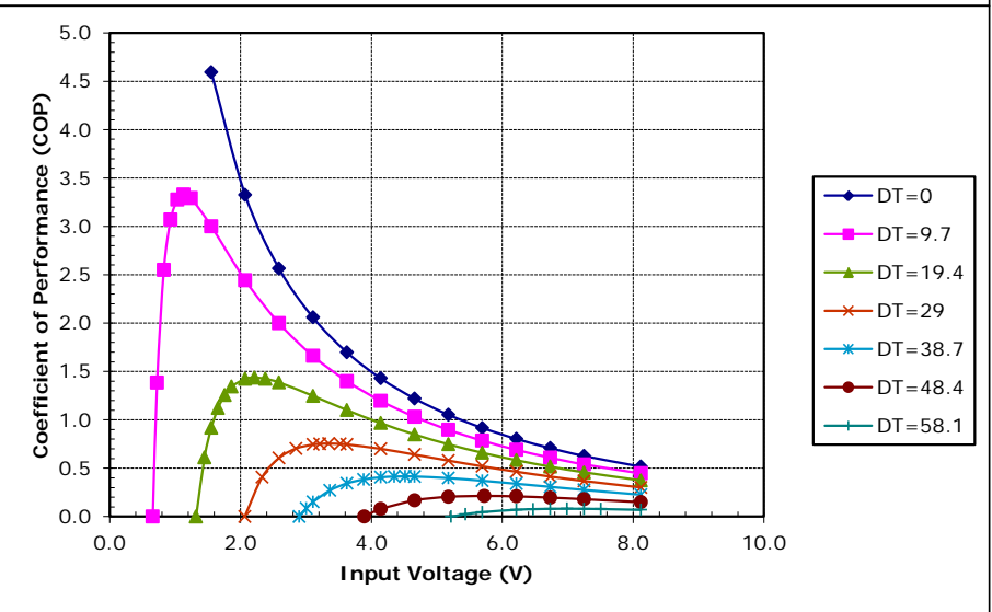
Potted TE-65-0.6-1.0 at a hot-side temperature of 30 °C
