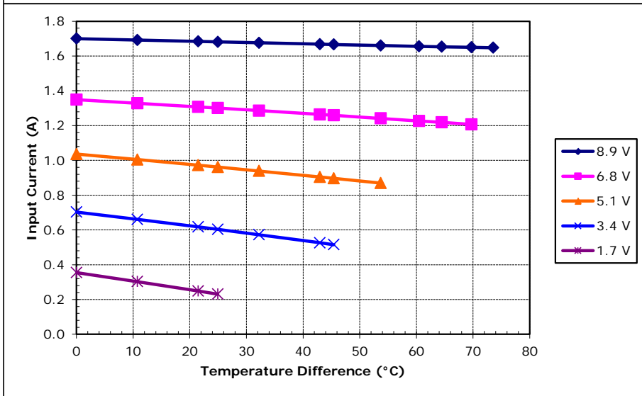
Potted TE-65-0.6-1.0 at a hot-side temperature of 50 °C
