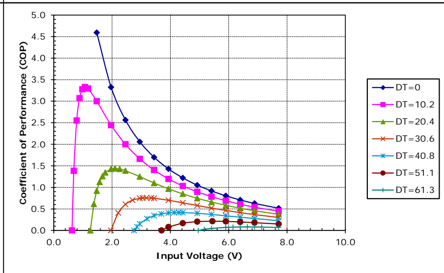
Unpotted TE-63-1.0-2.0 at a hot-side temperature of 30 °C
