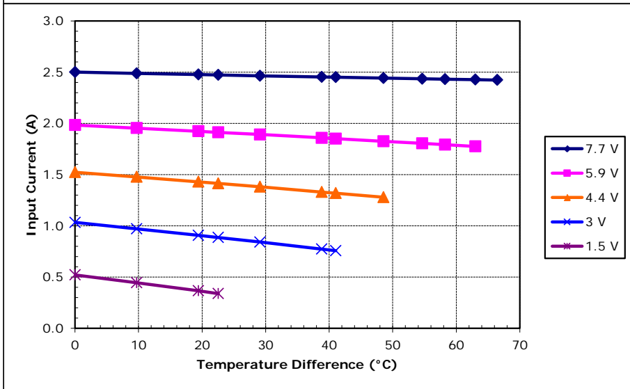
Potted TE-63-1.0-2.0 at a hot-side temperature of 30 °C
