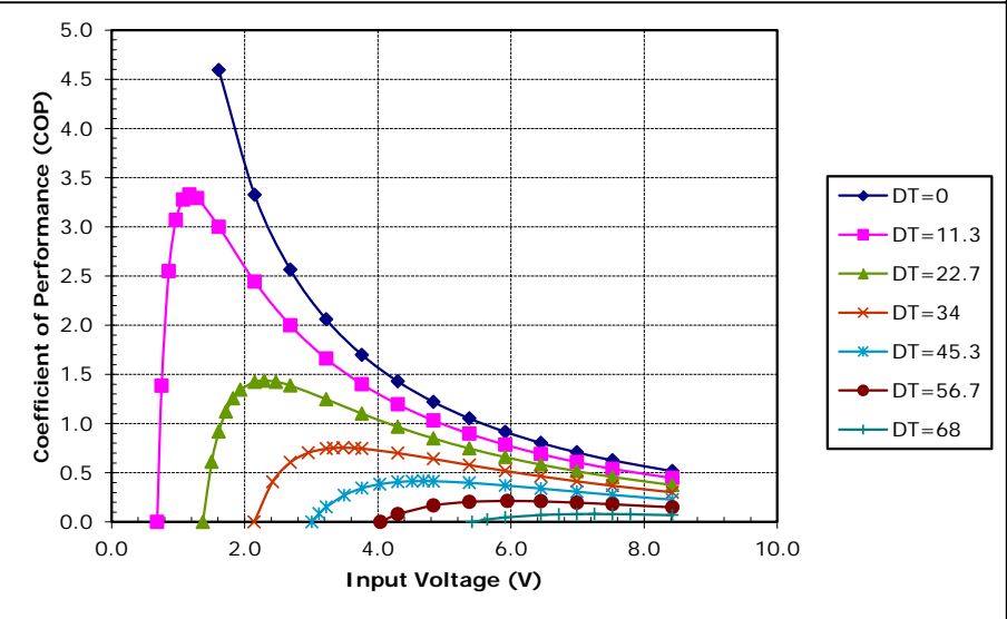
Unpotted TE-63-1.0-2.0 at a hot-side temperature of 50 °C
