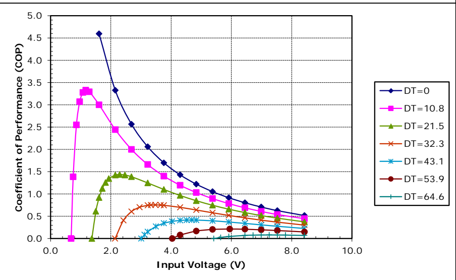
Potted TE-63-1.0-2.0 at a hot-side temperature of 50 °C
