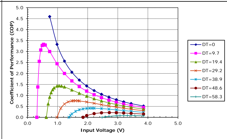
Unpotted TE-32-2.8-1.5 at a hot-side temperature of 30 °C
