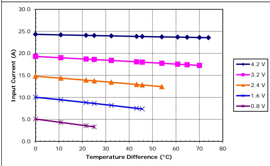
Unpotted TE-32-2.8-1.5 at a hot-side temperature of 50 °C
