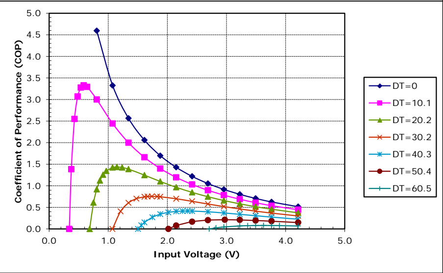
Potted TE-32-2.8-1.5 at a hot-side temperature of 50 °C
