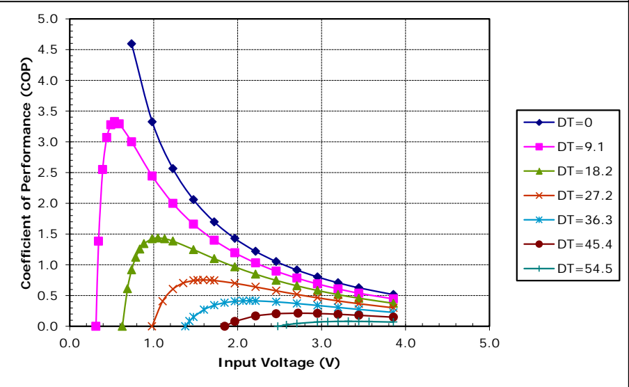
Potted TE-32-2.8-1.5 at a hot-side temperature of 30 °C
