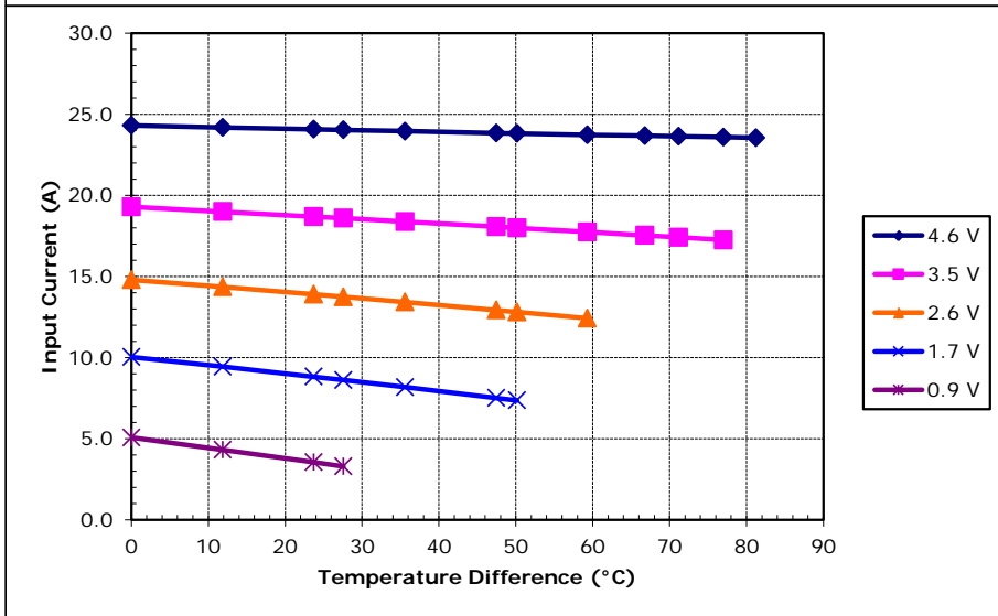
Unpotted TE-32-2.8-1.5 at a hot-side temperature of 70 °C
