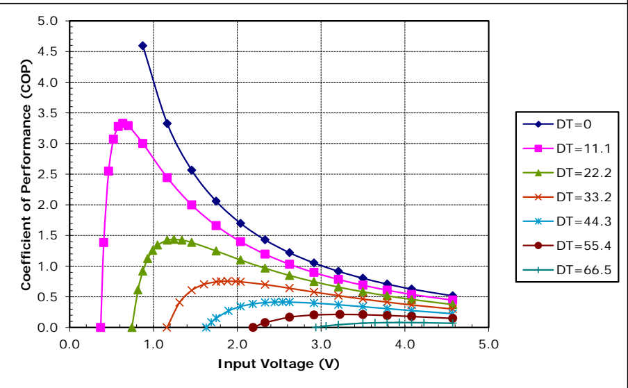
Potted TE-32-2.8-1.5 at a hot-side temperature of 70 °C
