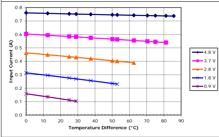
Unpotted TE-32-0.45-1.3 at a hot-side temperature of 70 °C
