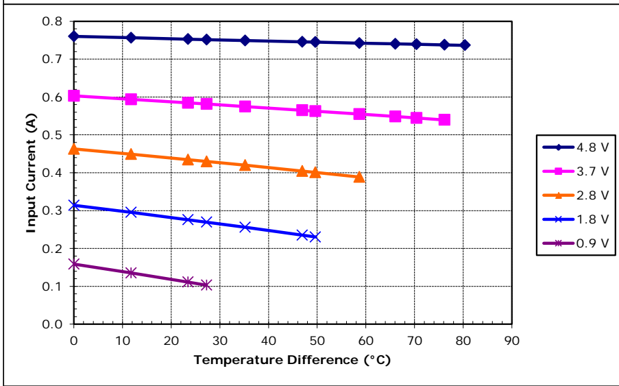
Potted TE-32-0.45-1.3 at a hot-side temperature of 70 °C
