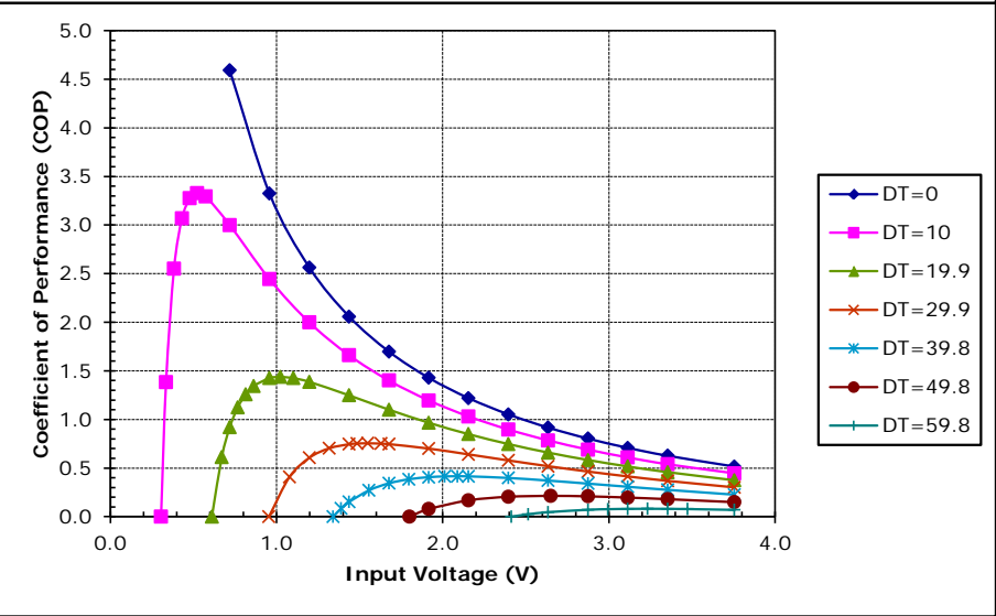
Unpotted TE-31-2.0-1.5 at a hot-side temperature of 30 °C
