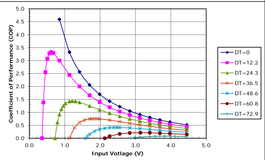
Unpotted TE-31-2.0-1.5 at a hot-side temperature of 70 °C
