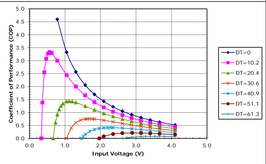
Potted TE-31-2.0-1.5 at a hot-side temperature of 50 °C
