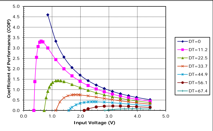
Potted TE-31-2.0-1.5 at a hot-side temperature of 70 °C
