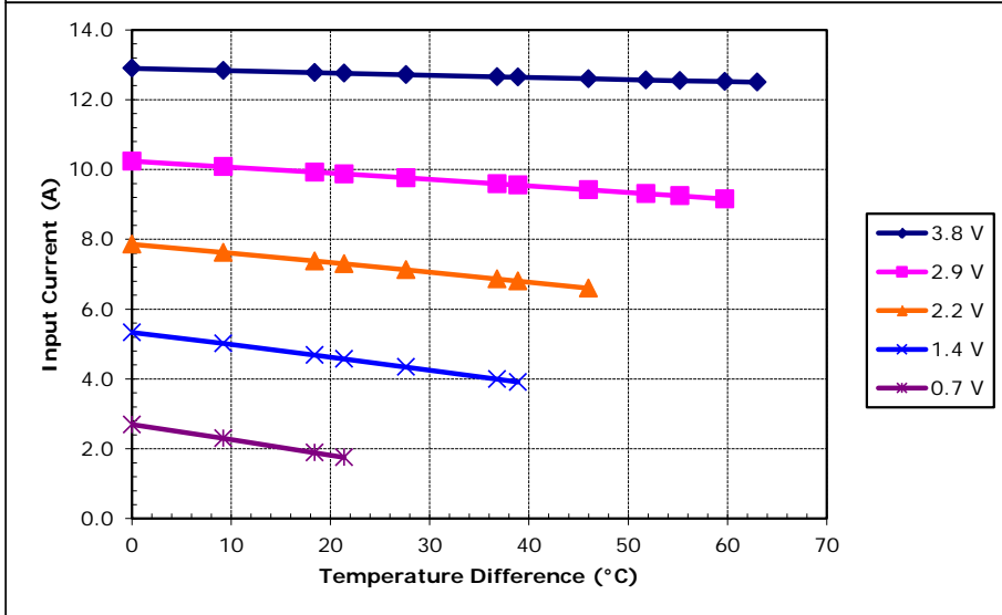
Potted TE-31-2.0-1.5 at a hot-side temperature of 30 °C
