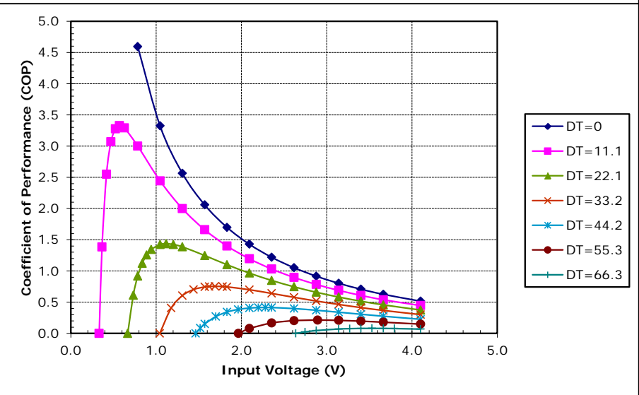
Unpotted TE-31-2.0-1.5 at a hot-side temperature of 50 °C
