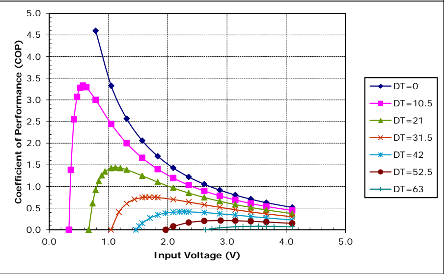
Potted TE-31-1.4-1.5 at a hot-side temperature of 50 °C
