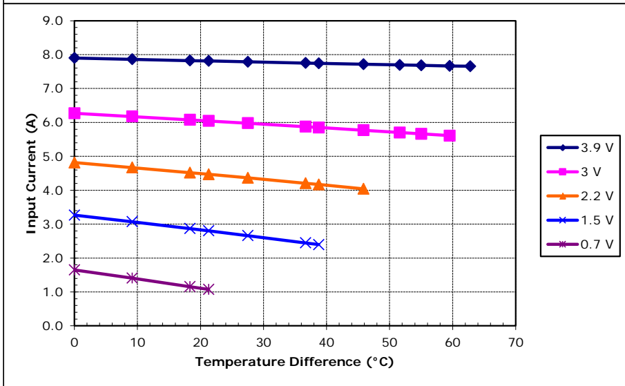
Potted TE-31-1.4-1.15 at a hot-side temperature of 30 °C
