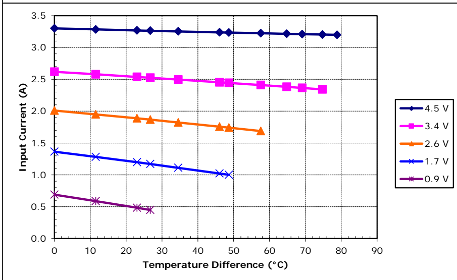
Potted TE-31-1.0-1.5 at a hot-side temperature of 70 °C
