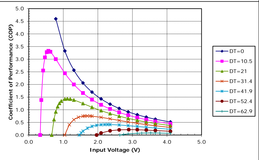
Potted TE-31-1.0-1.5 at a hot-side temperature of 50 °C
