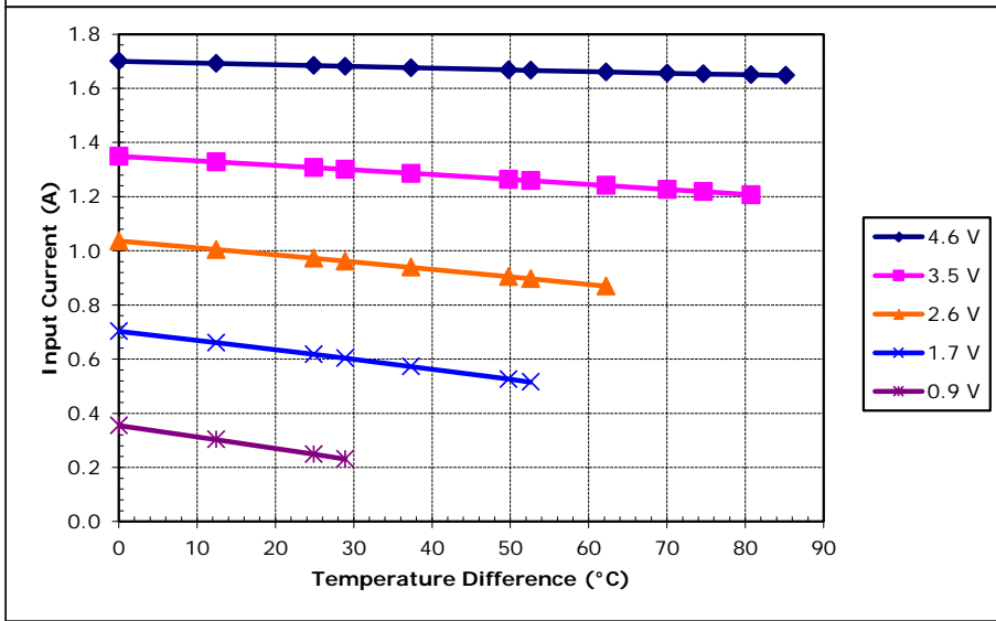
Unpotted TE-31-0.6-1.0 at a hot-side temperature of 70 °C
