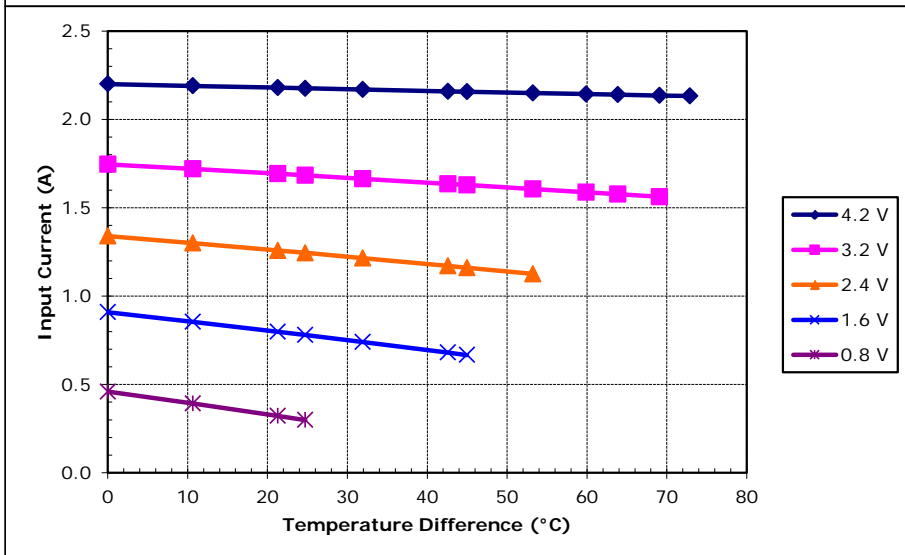
Potted TE-31-0.6-0.8 at a hot-side temperature of 50 °C
