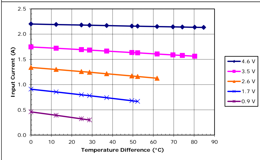
Unpotted TE-31-0.6-0.8 at a hot-side temperature of 70 °C
