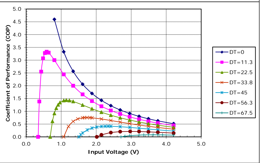
Unpotted TE-31-0.6-0.8 at a hot-side temperature of 50 °C
