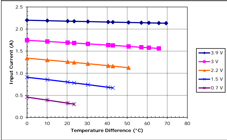
Unpotted TE-31-0.6-0.8 at a hot-side temperature of 30 °C
