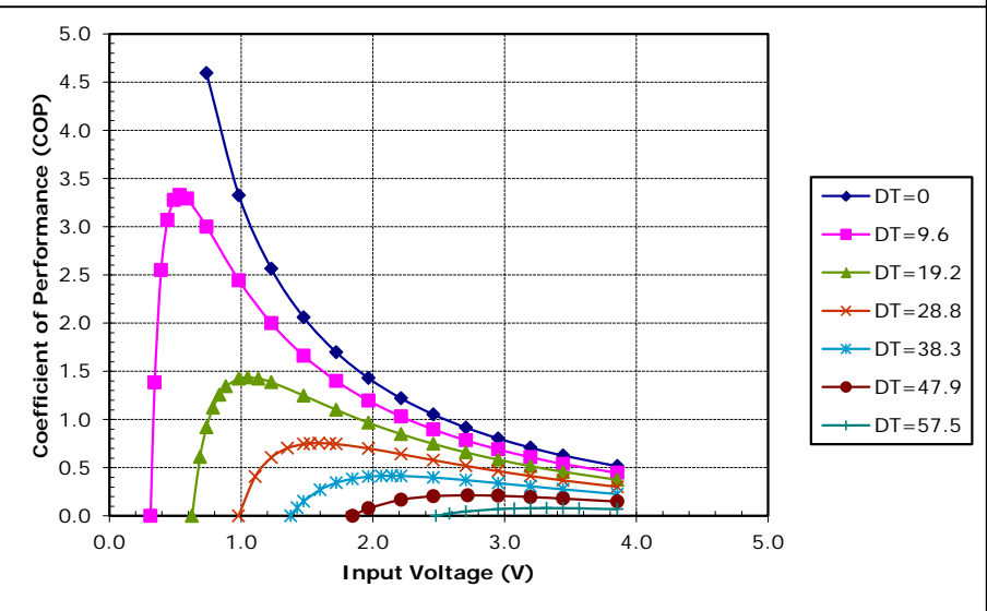
Potted TE-31-0.6-0.8 at a hot-side temperature of 30 °C
