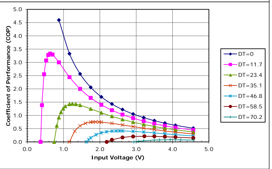
Potted TE-31-0.6-0.8 at a hot-side temperature of 70 °C
