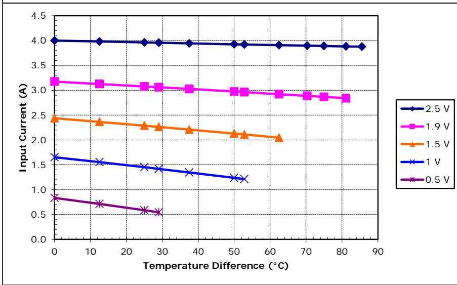
Unpotted TE-17-1.4-2.5 at a hot-side temperature of 70 °C
