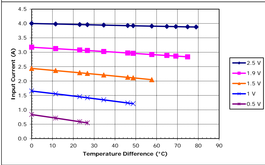
Potted TE-17-1.4-2.5 at a hot-side temperature of 70 °C
