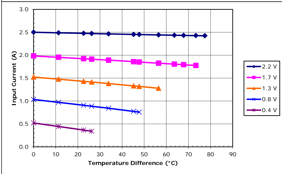
Unpotted TE-17-1.0-2.0 at a hot-side temperature of 50 °C
