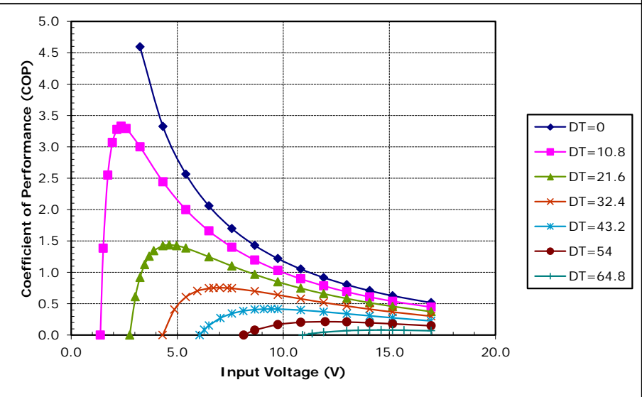
Unpotted TE-127-2.0-1.15 at a hot-side temperature of 50 °C
