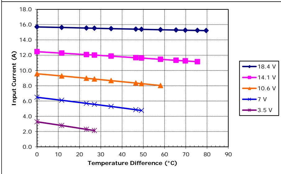
Potted TE-127-2.0-1.15 at a hot-side temperature of 70 °C
