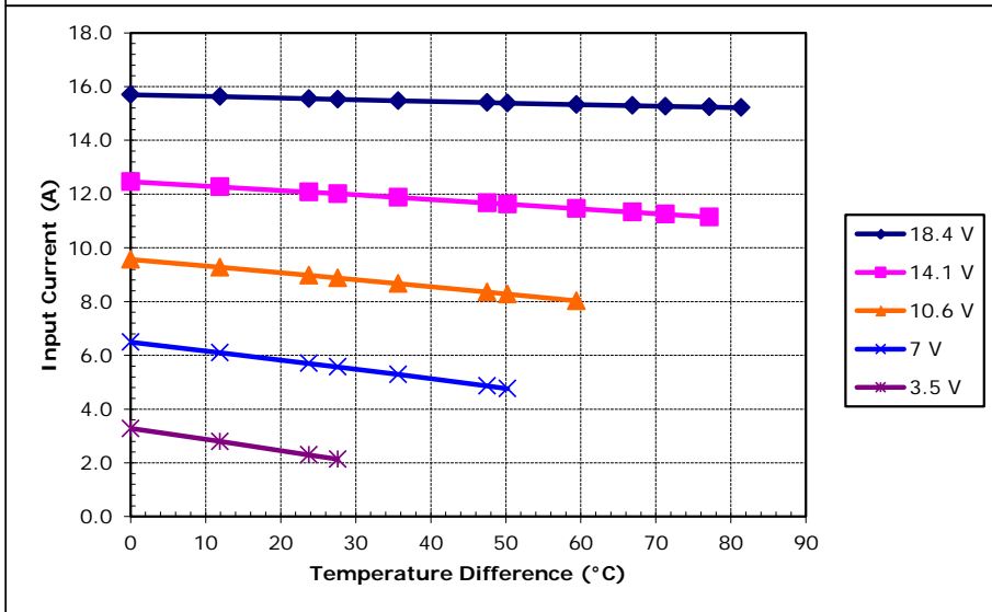
Unpotted TE-127-2.0-1.15 at a hot-side temperature of 70 °C
