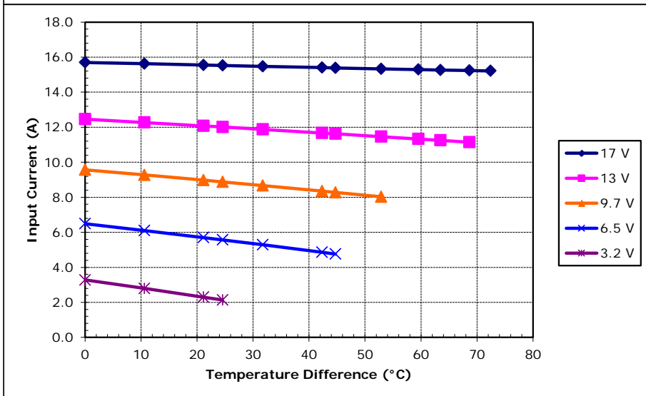
Potted TE-127-2.0-1.15 at a hot-side temperature of 50 °C
