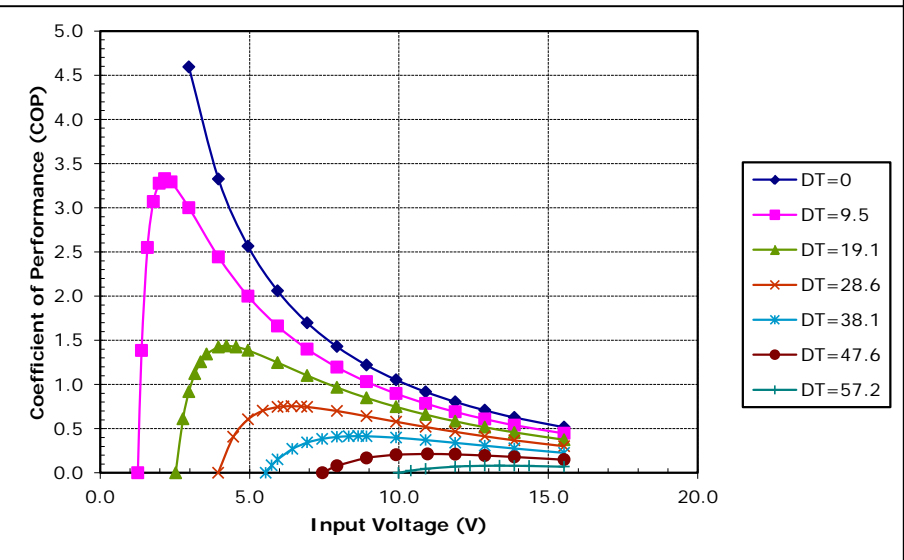
Potted TE-127-2.0-1.15 at a hot-side temperature of 30 °C
