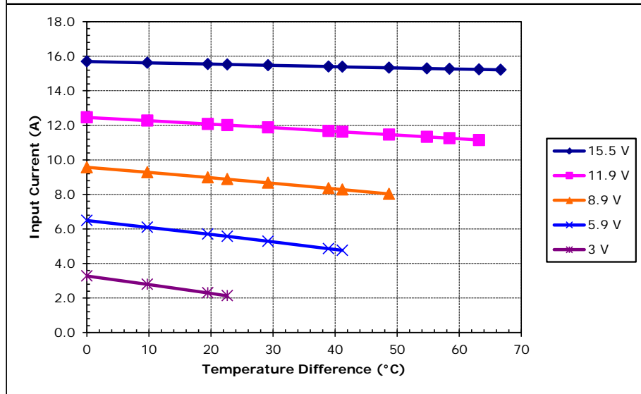
Unpotted TE-127-2.0-1.15 at a hot-side temperature of 30 °C
