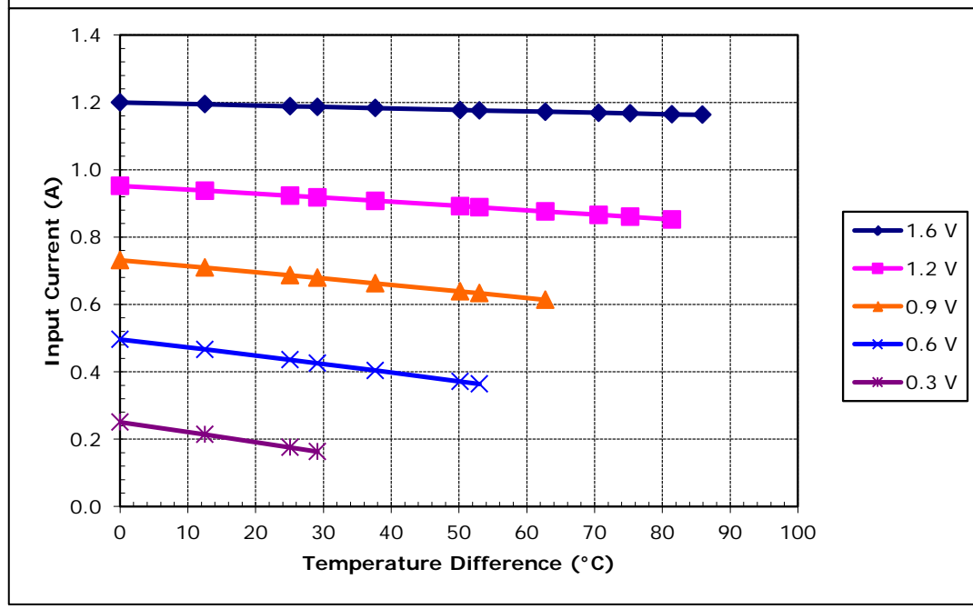
Unpotted TE-11-0.6-1.5 at a hot-side temperature of 70 °C
