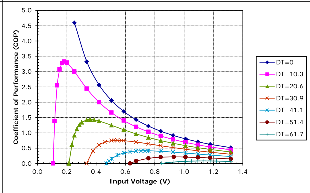
Unpotted TE-11-0.6-1.5 at a hot-side temperature of 30 °C
