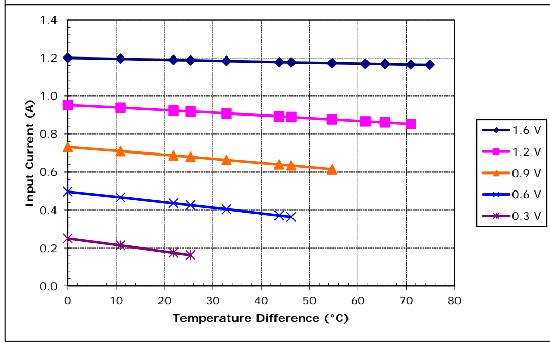
Potted TE-11-0.6-1.5 at a hot-side temperature of 70 °C
