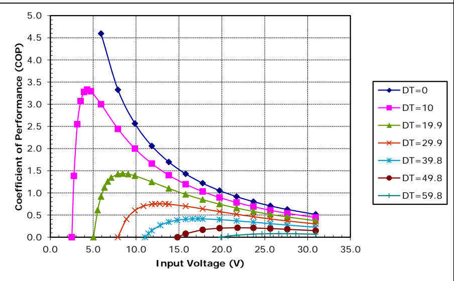
Potted RD-253-1.4-1.5 at a hot-side temperature of 30 °C
