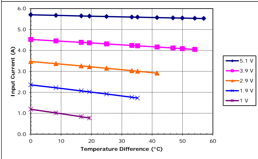
Potted CH-41-1.0-0.8 at a hot-side temperature of 30 °C
