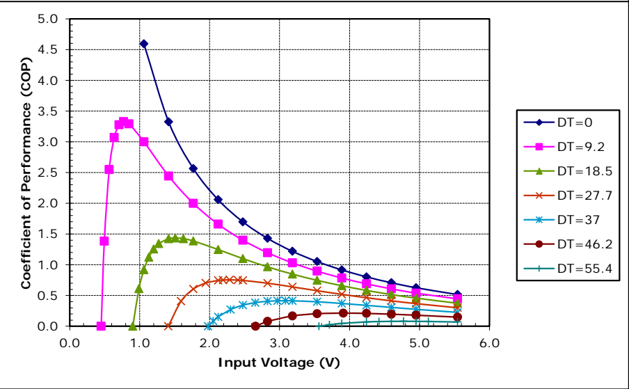
Potted CH-41-1.0-0.8 at a hot-side temperature of 50 °C
