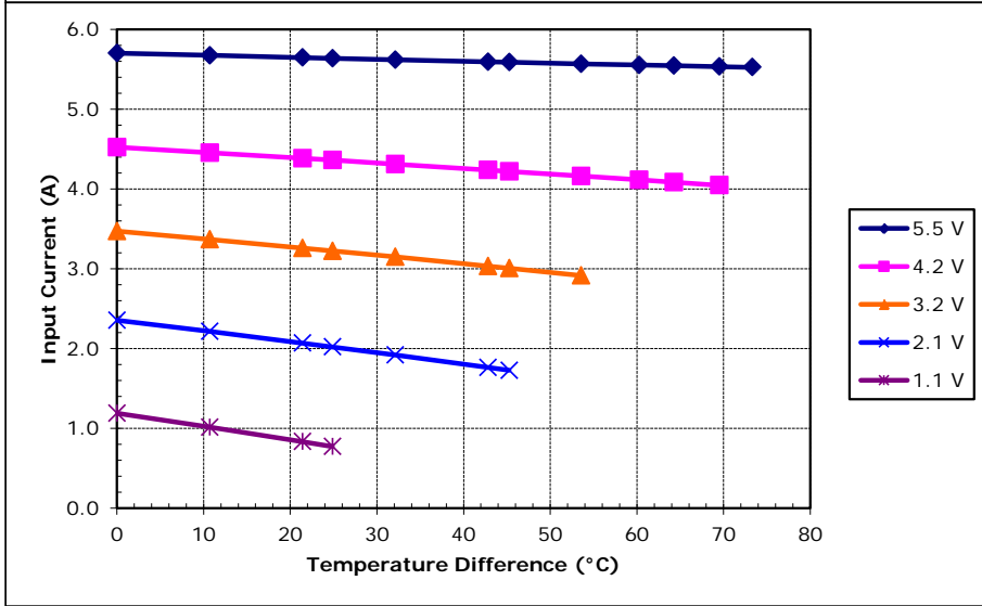
Unpotted CH-41-1.0-0.8 at a hot-side temperature of 50 °C
