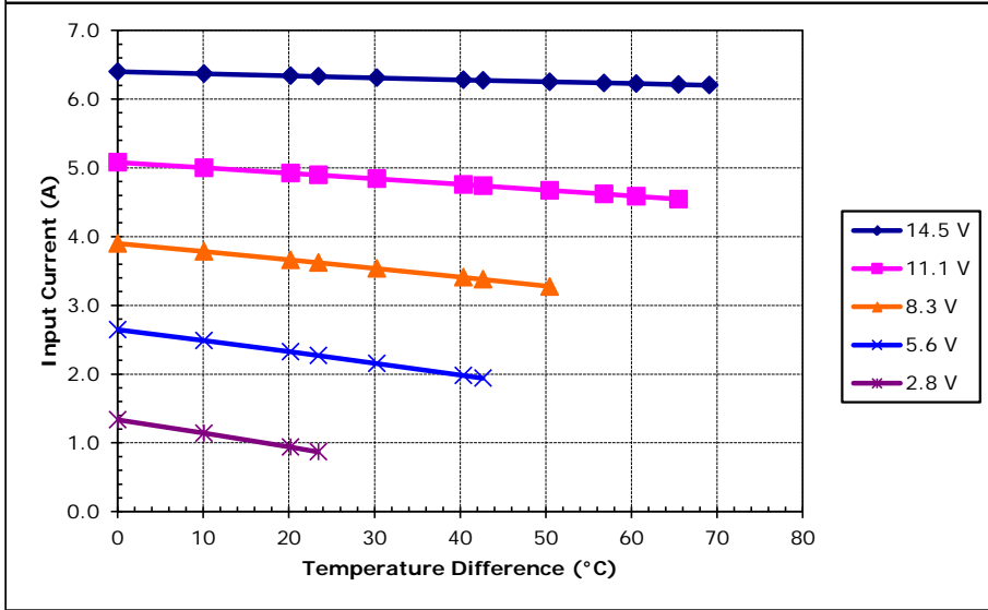
Unpotted CH-119-1.4-1.5 at a hot-side temperature of 30 °C
