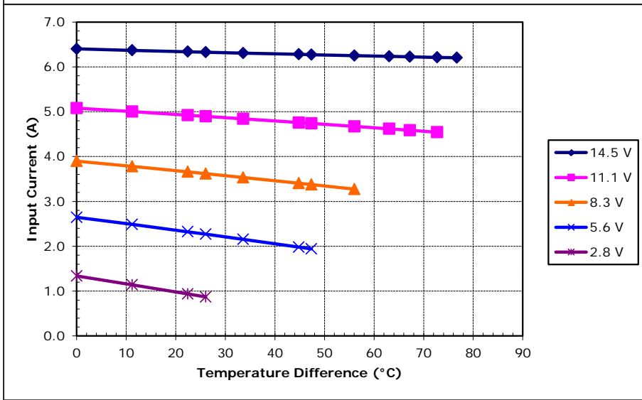
Unpotted CH-109-1.4-1.5 at a hot-side temperature of 50 °C
