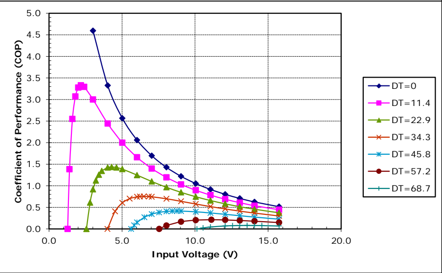
Potted CH-109-1.4-1.5 at a hot-side temperature of 70 °C
