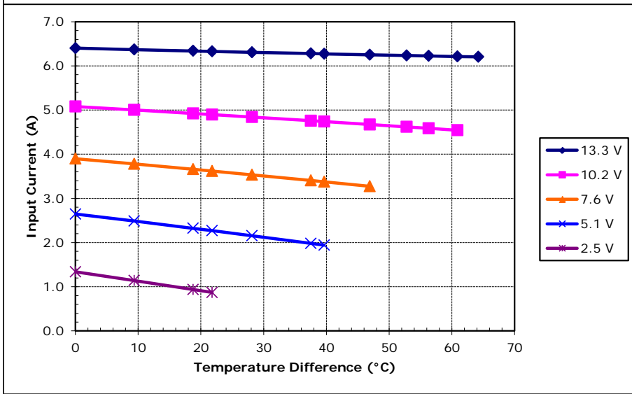
Potted CH-109-1.4-1.5 at a hot-side temperature of 30 °C
